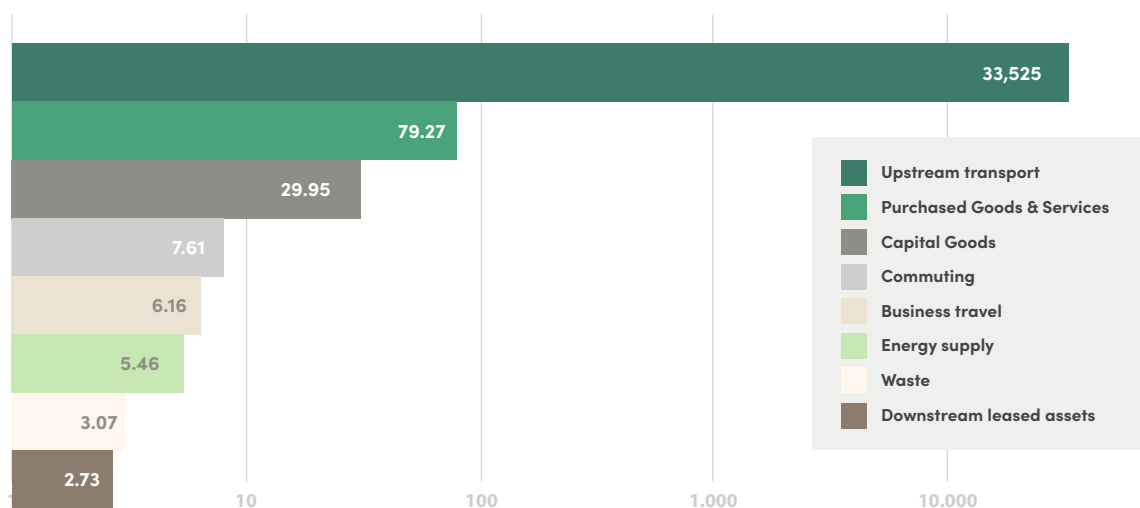
Figure: Overview of emissions by category (top: all categories, bottom: excluding upstream transport)
